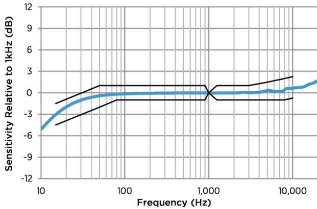
Figure 3: Typical Free Field Magnitude Response and Masks
