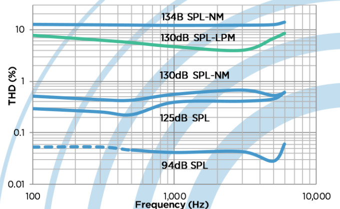
Figure 6: Typical THD vs Input Frequency
