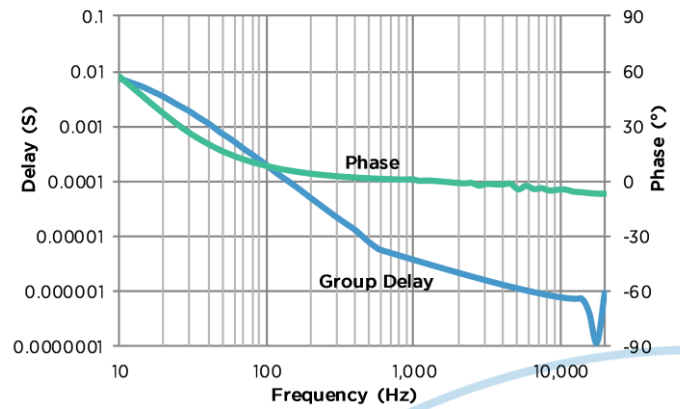
Figure 5: Typical Phase Response and Group Delay
