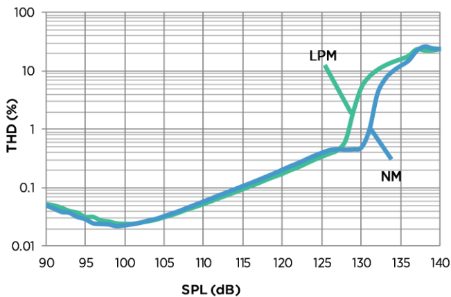
Figure 4: Typical THD vs Input SPL
